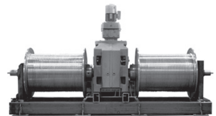
Dual Drum Hoist with 3 fpm (.015 m/s), 13,500 lb (6,123 kg) lifting capacity
