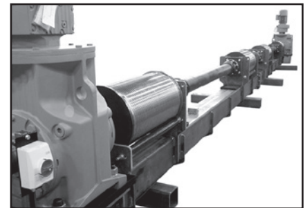
Custom hoist with 34,000 lb (15,422 kg) lifting capacity
